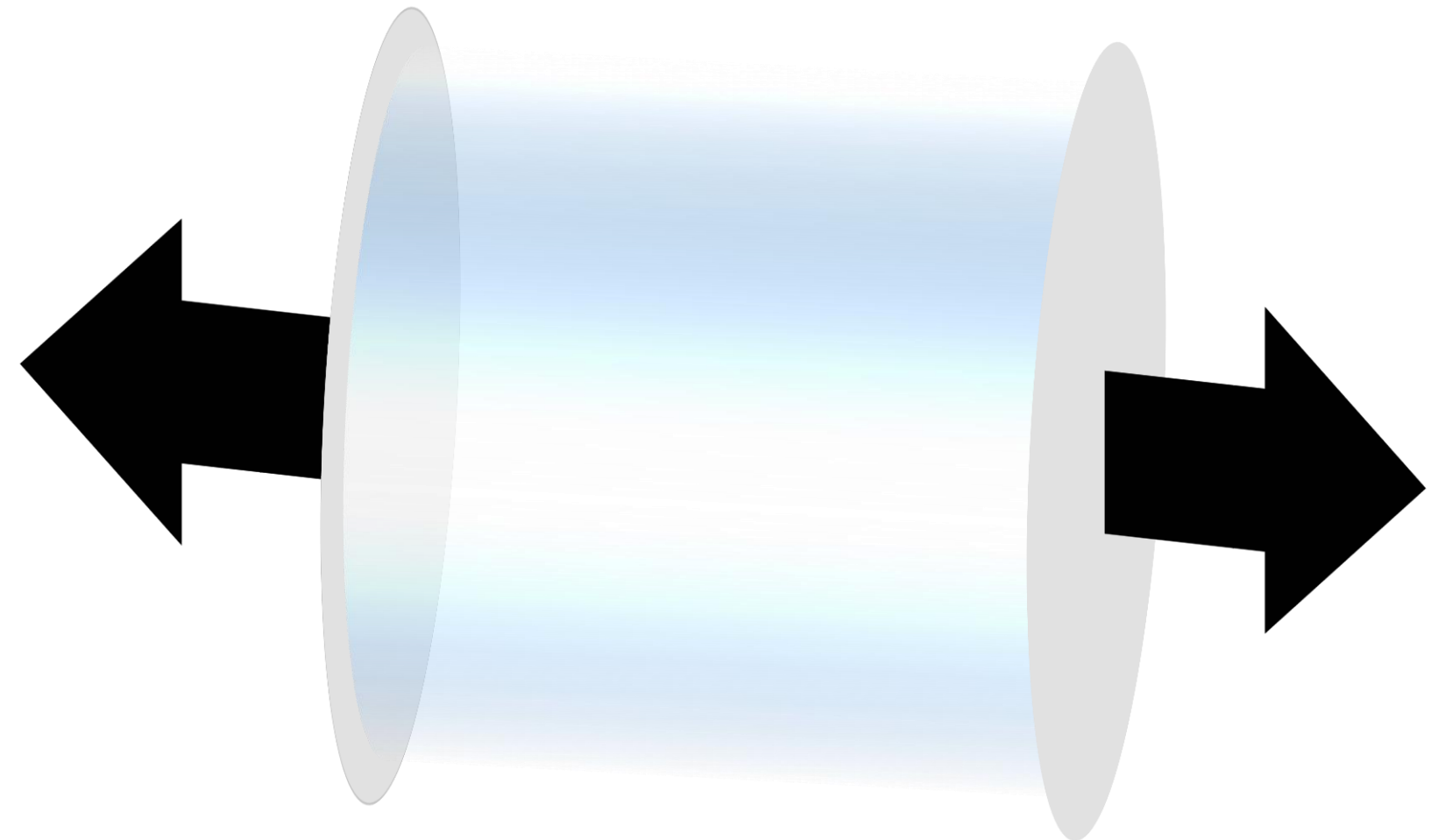
Quark Gluon Plasma( \tau \gtrsim 0.6 fm/c)
